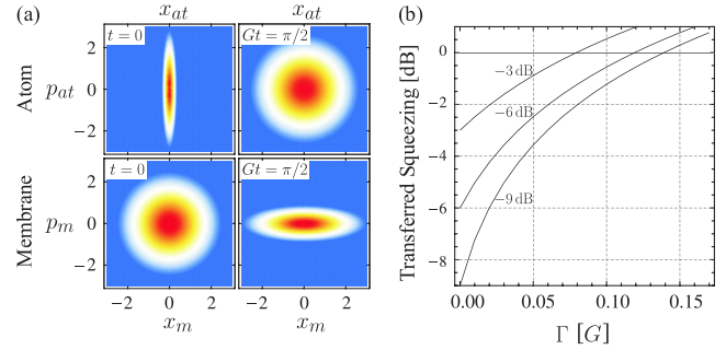
FIG. 2 (color online). (a) Wigner functions of atom and membrane (upper and lower panels, respectively). At t = 0 (left-hand panels) the atom is in a squeezed state (9 dB) and the membrane in a thermal state with a mean number of phonons \bar{n} = 5 . An exact solution of the equation of motion (2) with losses \Gamma = \Gamma_c, \Gamma_m, \Gamma_{at} at rate \Gamma = 0.1G shows that after a time Gt = \frac{\pi}{2} (right-hand panels) the states are exchanged, up to a trivial rotation in phase space by 90^\circ . (b) Squeezing transferred to membrane (maximized over time), versus loss rate \Gamma , for the indicated values of initial atomic position fluctuations.
