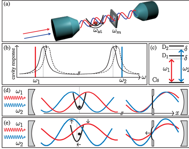
FIG. 1 (color online). (a) Strong coupling of the motion of a single atom to a vibrational degree of freedom of a micron-sized membrane can be achieved in a two mode cavity (for details see text). (b) Cavity response as a function of frequency. Two cavity modes are driven by two lasers of frequencies \omega_1 and \omega_2 , with red and blue detuning, respectively. (c) The two frequencies drive two atomic transitions, e.g., the D_{1,2} lines of Cs, both with red detuning, causing ac Stark shift of the ground state. (d) (Left-hand side) The atom is trapped in the potential from the two optical lattices. (Right-hand side) The membrane is placed at a point of steepest slope of the intensity profiles. (e) A small displacement of the membrane will shift the cavity resonances [cf. dashed line in (b)] resulting in a spatial shift of the trap potential for the atom, and thus an effective linear atom-membrane coupling as in Eq. (1).
